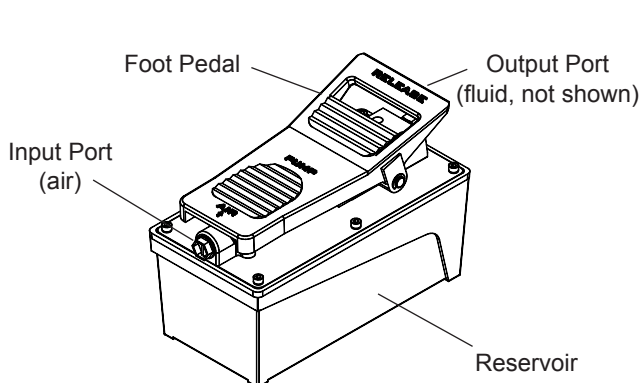
Figure 1 - Model 22903 Components
