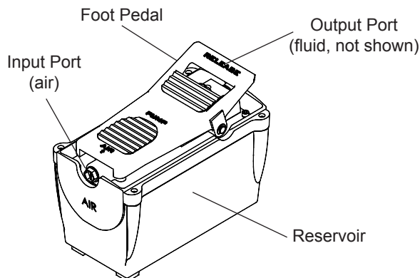
Figure 2 - Model 22905 components
