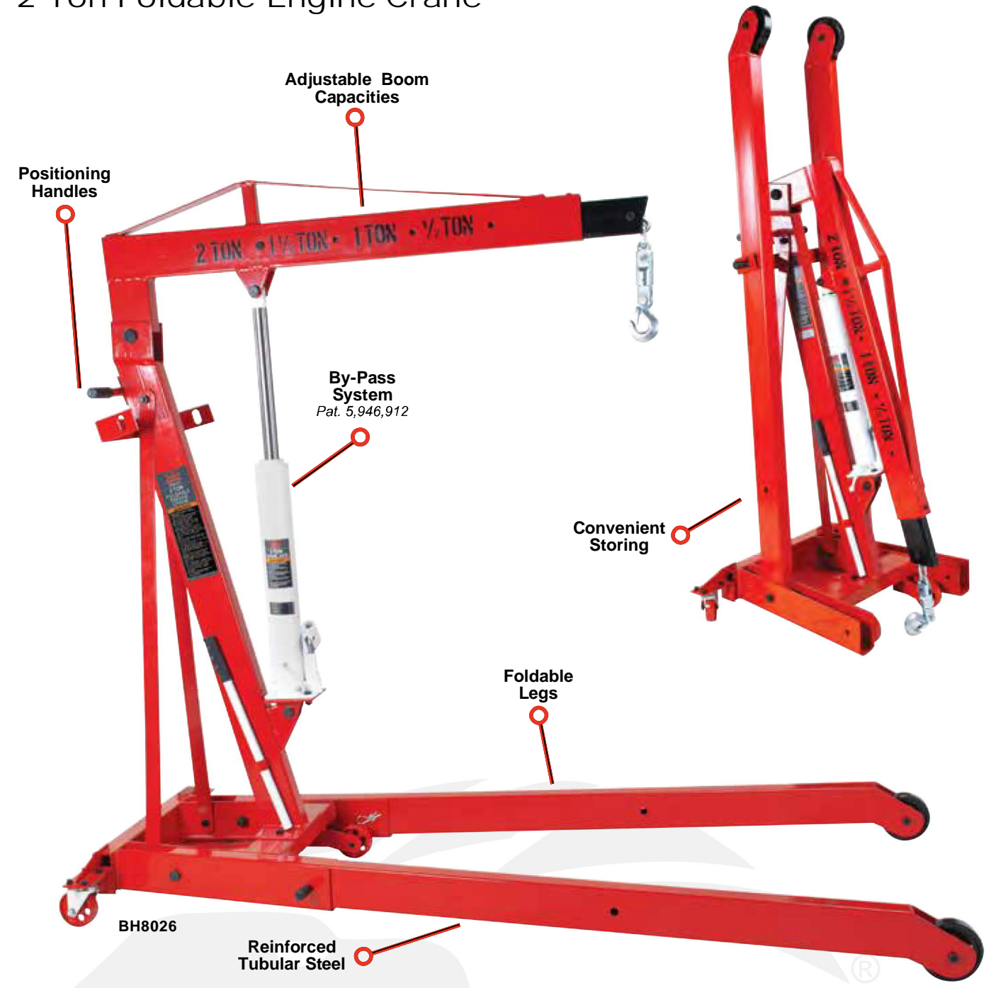
2 Ton Foldable Engine Crane
